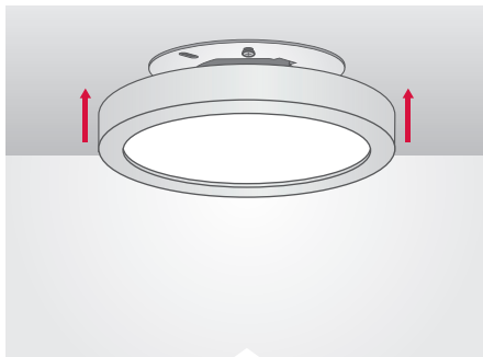
STEP 6: Push and feed all wires up into junction box as you raise the fixture into place. For wet location usage, seal/caulk the edge of the fixture to the ceiling with waterproof sealant.
