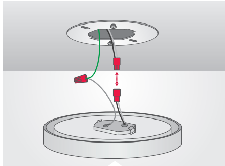
STEP 4: Make ground connection. Next simply „click“ the two sides of the orange wire connector together.
