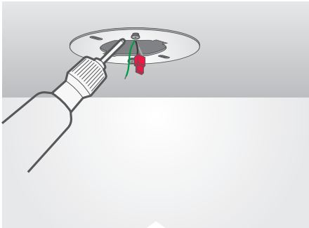
STEP 3: Attach the bracket to junction box using 2 screws (provided). Pull the AC cable with connector through the bracket center hole.
